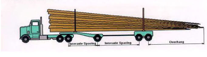
Medium Spread Single Axle Jeep Logger
