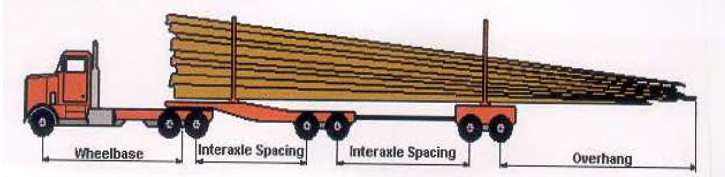
Tandem Axle Jeep Logger
