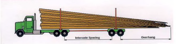
Tandem Axle Jeep Logger
