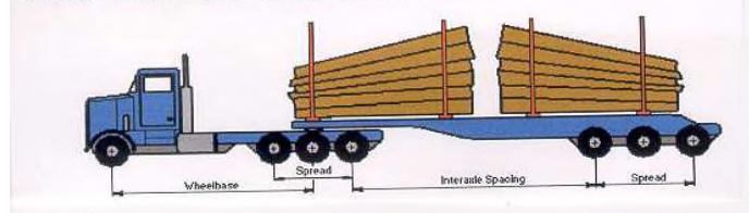
Tridem Drive Truck – Tridem Semi Trailer
